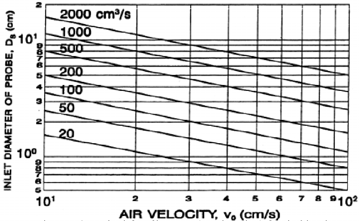
Figure C.1. Probe inlet diameters (metric units) for isokinetic sampling, v = v_0 (volumetric flow rates shown parametrically)
