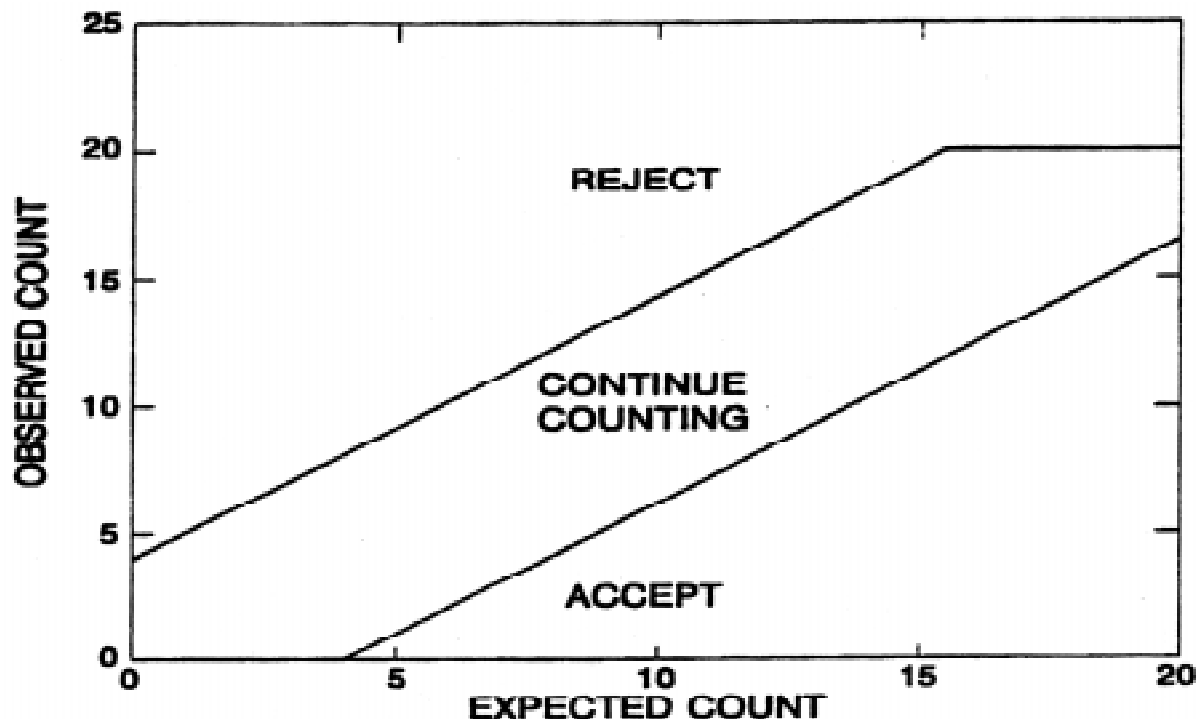
Figure F.1. Observed count, C , vs. expected count, E , for sequential sampling. The labels delineate those regions where the cumulative observed count indicates that the air either exceeds the class limit or U descriptor (REJECT), meets the class limit or U descriptor (ACCEPT), or is indeterminate (CONTINUE COUNTING).
