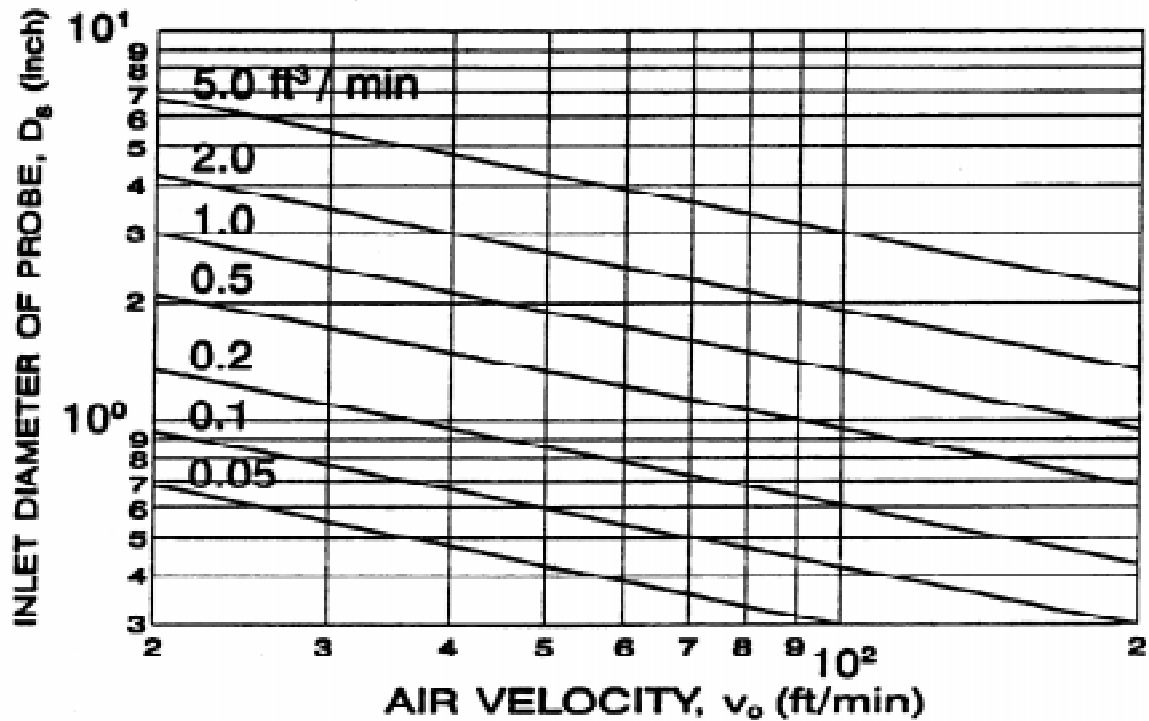
Figure C.2. Probe inlet diameters (English units) for isokinetic sampling, v = v_0 (volumetric flow rates shown parametrically).
