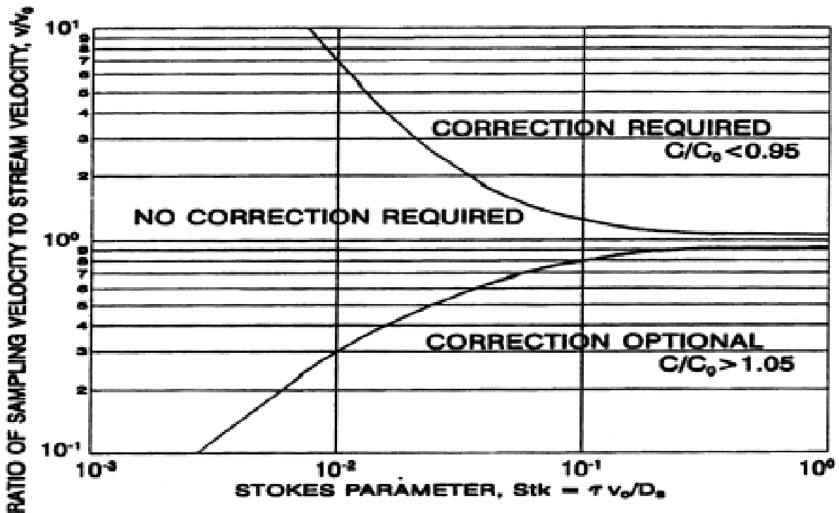
Figure C.3: Contours of sampling bias; C/C_0 = 0.95 to 1.05
